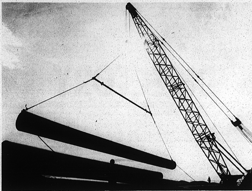
AN 80-FOOT SECTION of pipe for the trans Alaska pipeline is stacked at a temporary storage yard north of the Yukon River. The 48-inch diameter pipe for the pipeline, which has been stored in Valdez, Fairbanks and Prudhoe Bay for almost five years, is being transported to similar yards along the 800-mile-long pipeline route.
